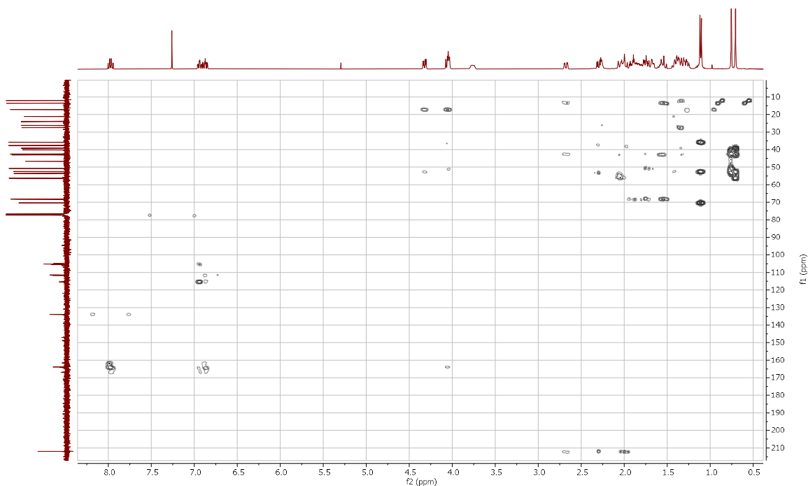
Fig. S20. 2D ^1\text{H} - ^{13}\text{C} HMBC NMR Spectrum of 2\alpha,3\alpha -Dihydroxy-6-oxo-23,24-dinor- 5\alpha -cholan-22-yl-(2,4-difluoro)-benzoate ( 18 ).
