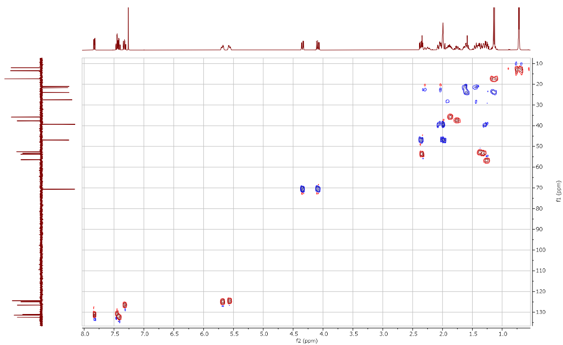
Fig. S9. 2D ^1\text{H} - ^{13}\text{C} HSQC NMR Spectrum of 6-Oxo-23,24-dinor-5 \alpha -Cholan-2-en-22-yl-(2-chloro)-benzoate (23).
