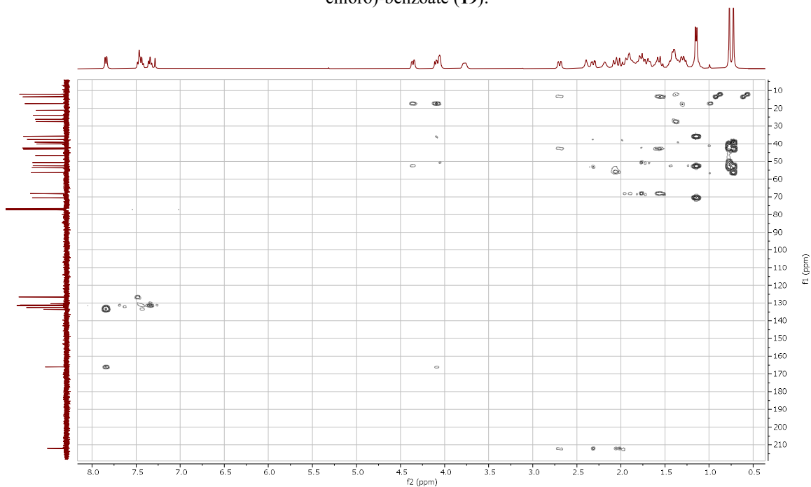
Fig. S26. 2D ^1\text{H} - ^{13}\text{C} HMBC NMR Spectrum of 2\alpha,3\alpha -Dihydroxy-6-oxo-23,24-dinor- 5\alpha -cholan-22-yl-(2-chloro)-benzoate ( 19 ).
