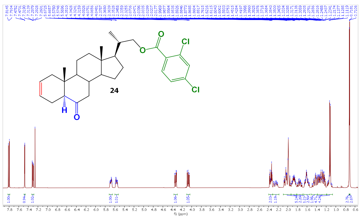
Fig. S11. ^1\text{H} NMR Spectrum of 6-Oxo-23,24-dinor-5 \alpha -Cholan-2-en-22-yl-(2,4-dichloro)-benzoate (24).
