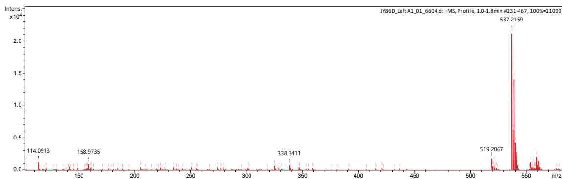
Fig. S33. HRMS spectrum of 2 \alpha ,3 \alpha -Dihydroxy-6-oxo-23,24-dinor-5 \alpha -cholan-22-yl-(2,4-dichloro)-benzoate ( 20 ).
