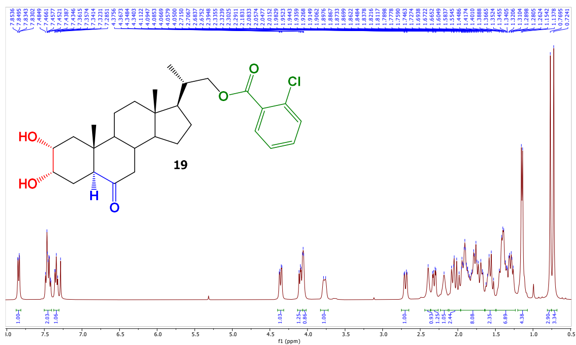
Fig. S22. 1 H NMR Spectrum of 2 \alpha ,3 \alpha -Dihydroxy-6-oxo-23,24-dinor-5 \alpha -cholan-22-yl-(2-chloro)-benzoate (19).
