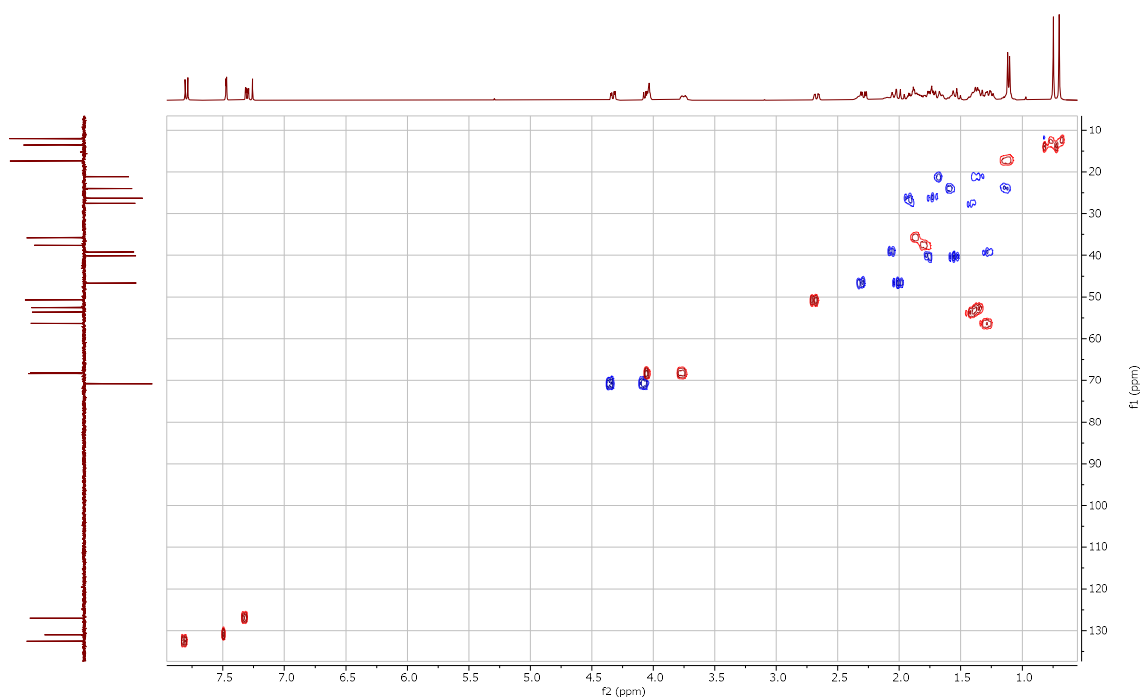
Fig. S31. 2D ^1\text{H} - ^{13}\text{C} HSQC NMR Spectrum of 2\alpha,3\alpha -Dihydroxy-6-oxo-23,24-dinor- 5\alpha -cholan-22-yl-(2,4-dichloro)-benzoate ( 20 ).
