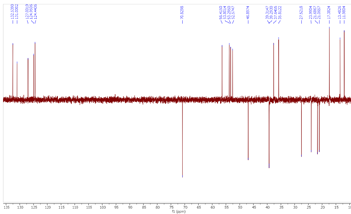
Fig. S13. ^{13}\text{C} DEPT-135 NMR Spectrum of 6-Oxo-23,24-dinor-5 \alpha -Cholan-2-en-22-yl-(2,4-dichloro)-benzoate (24).
