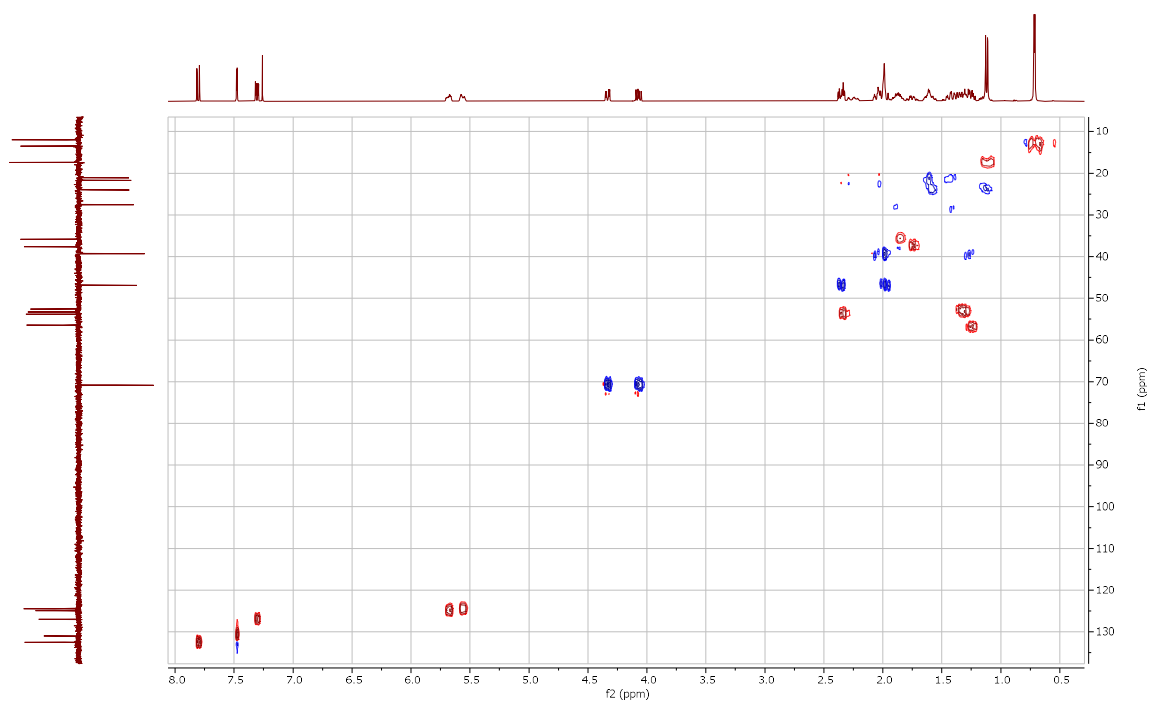
Fig. S14. 2D ^1\text{H} - ^{13}\text{C} HSQC NMR Spectrum of 6-Oxo-23,24-dinor-5 \alpha -Cholan-2-en-22-yl-(2,4-dichloro)-benzoate (24).
