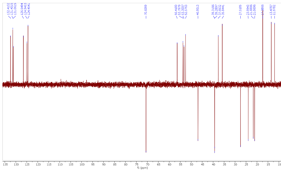
Fig. S8. ^{13}\text{C} DEPT-135 NMR Spectrum of 6-Oxo-23,24-dinor-5 \alpha -Cholan-2-en-22-yl-(2-chloro)-benzoate ( 23 ).
