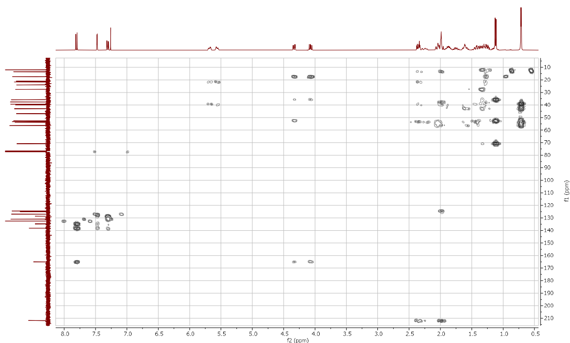
Fig. S15. 2D ^1\text{H} - ^{13}\text{C} HMBC NMR Spectrum of 6-Oxo-23,24-dinor-5 \alpha -Cholan-2-en-22-yl-(2,4-dichloro)-benzoate ( 24 ).
