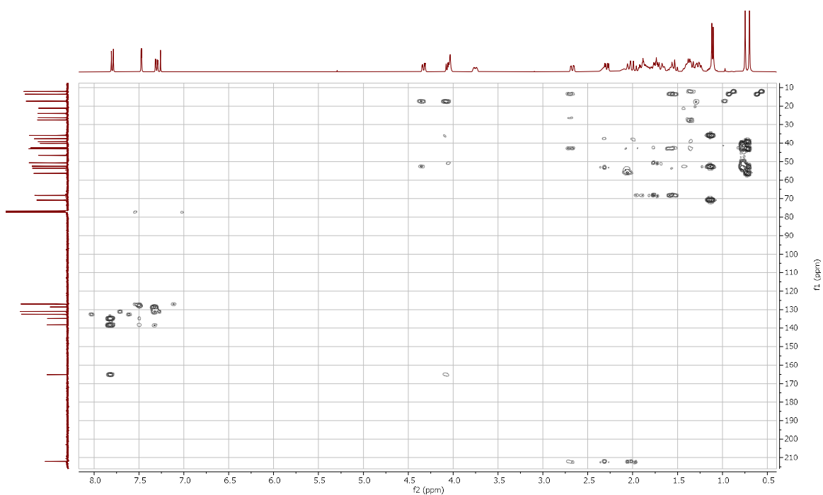
Fig. S32. 2D ^1\text{H} - ^{13}\text{C} HMBC NMR Spectrum of 2\alpha,3\alpha -Dihydroxy-6-oxo-23,24-dinor- 5\alpha -cholan-22-yl-(2,4-dichloro)-benzoate ( 20 ).
