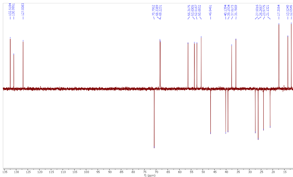
Fig. S30. ^{13}\text{C} DEPT-135 NMR Spectrum of 2\alpha,3\alpha -Dihydroxy-6-oxo-23,24-dinor- 5\alpha -cholan-22-yl-(2,4-dichloro)-benzoate ( 20 ).
