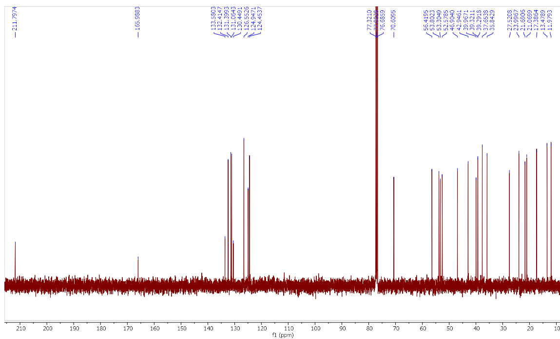
Fig. S7. ^{13}\text{C} NMR Spectrum of 6-Oxo-23,24-dinor-5 \alpha -Cholan-2-en-22-yl-(2-chloro)-benzoate ( 23 ).
