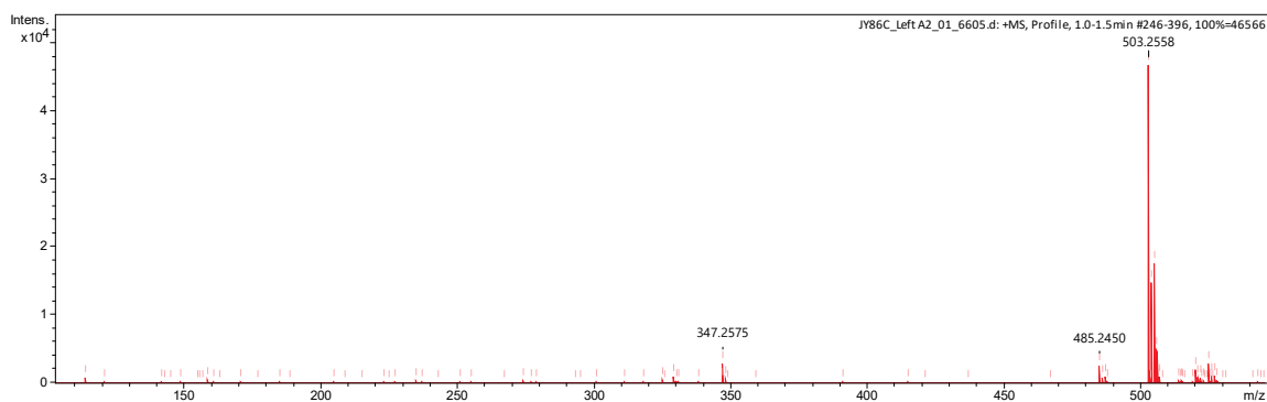
Fig. S21. HRMS spectrum of 2 \alpha ,3 \alpha -Dihydroxy-6-oxo-23,24-dinor-5 \alpha -cholan-22-yl-(2,4-difluoro)-benzoate (18).
