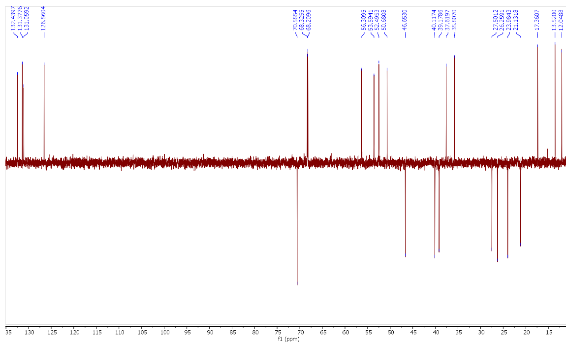
Fig. S24. ^{13}\text{C} DEPT-135 NMR Spectrum of 2\alpha,3\alpha -Dihydroxy-6-oxo-23,24-dinor- 5\alpha -cholan-22-yl-(2-chloro)-benzoate ( 19 ).
