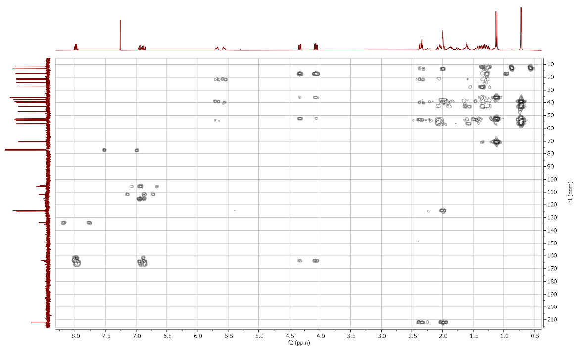
Fig. S5. 2D ^1\text{H} - ^{13}\text{C} HMBC Spectrum of 6-Oxo-23,24-dinor-5 \alpha -Cholan-2-en-22-yl-(2,4-difluoro)-benzoate ( 22 ).
