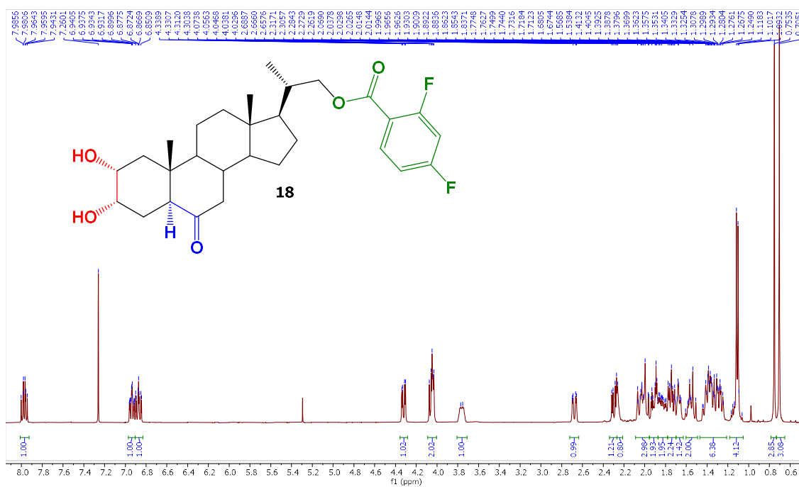
Fig. S16. ^1\text{H} NMR Spectrum of 2 \alpha ,3 \alpha -Dihydroxy-6-oxo-23,24-dinor-5 \alpha -cholan-22-yl-(2,4-difluoro)-benzoate ( 18 ).
