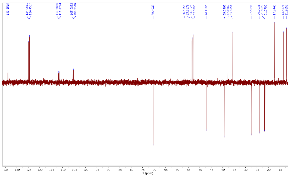
Fig. S3. ^{13}\text{C} DEPT-135 NMR Spectrum of 6-Oxo-23,24-dinor-5 \alpha -Cholan-2-en-22-yl-(2,4-difluoro)-benzoate (22).
