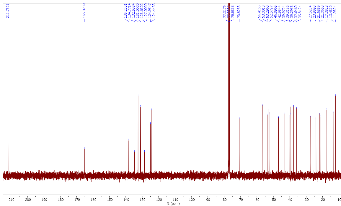
Fig. S12. ^{13}\text{C} NMR Spectrum of 6-Oxo-23,24-dinor-5 \alpha -Cholan-2-en-22-yl-(2,4-dichloro)-benzoate (24).
