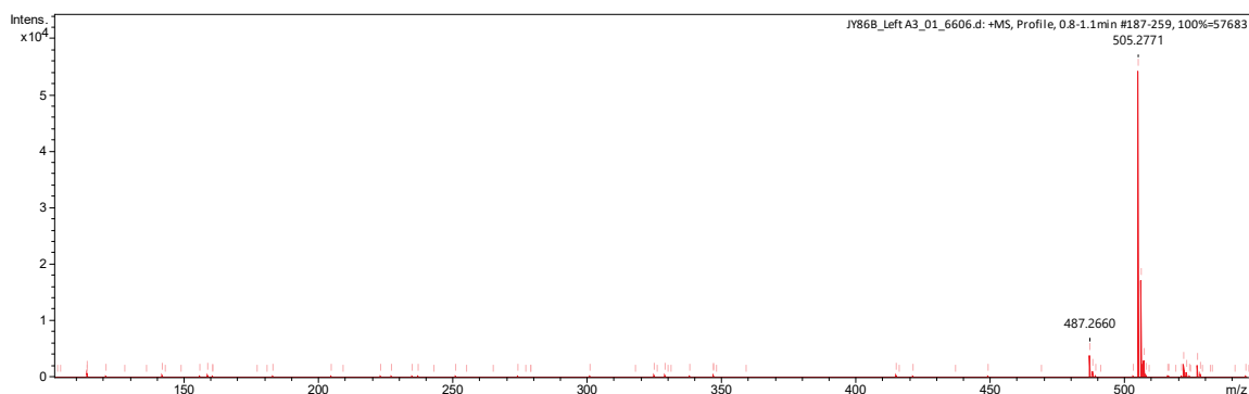
Fig. S27. HRMS spectrum of 2 \alpha ,3 \alpha -Dihydroxy-6-oxo-23,24-dinor-5 \alpha -cholan-22-yl-(2-chloro)-benzoate ( 19 ).
