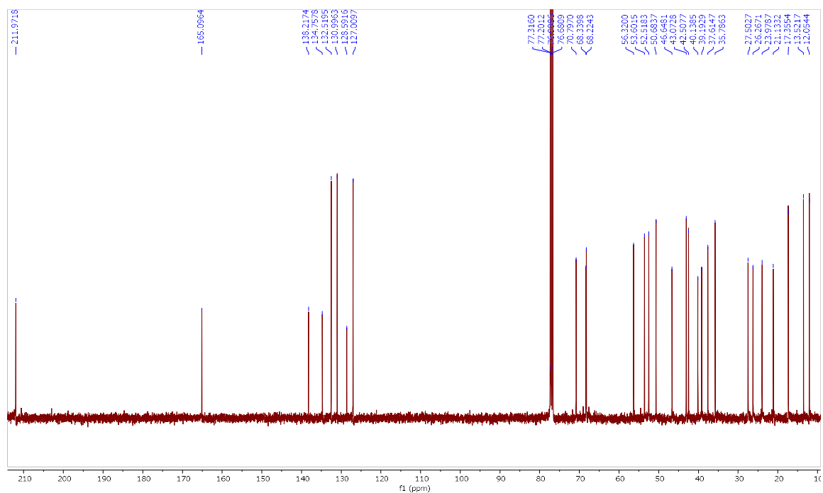
Fig. S29. ^{13}\text{C} NMR Spectrum of 2\alpha,3\alpha -Dihydroxy-6-oxo-23,24-dinor- 5\alpha -cholan-22-yl-(2,4-dichloro)-benzoate ( 20 ).
