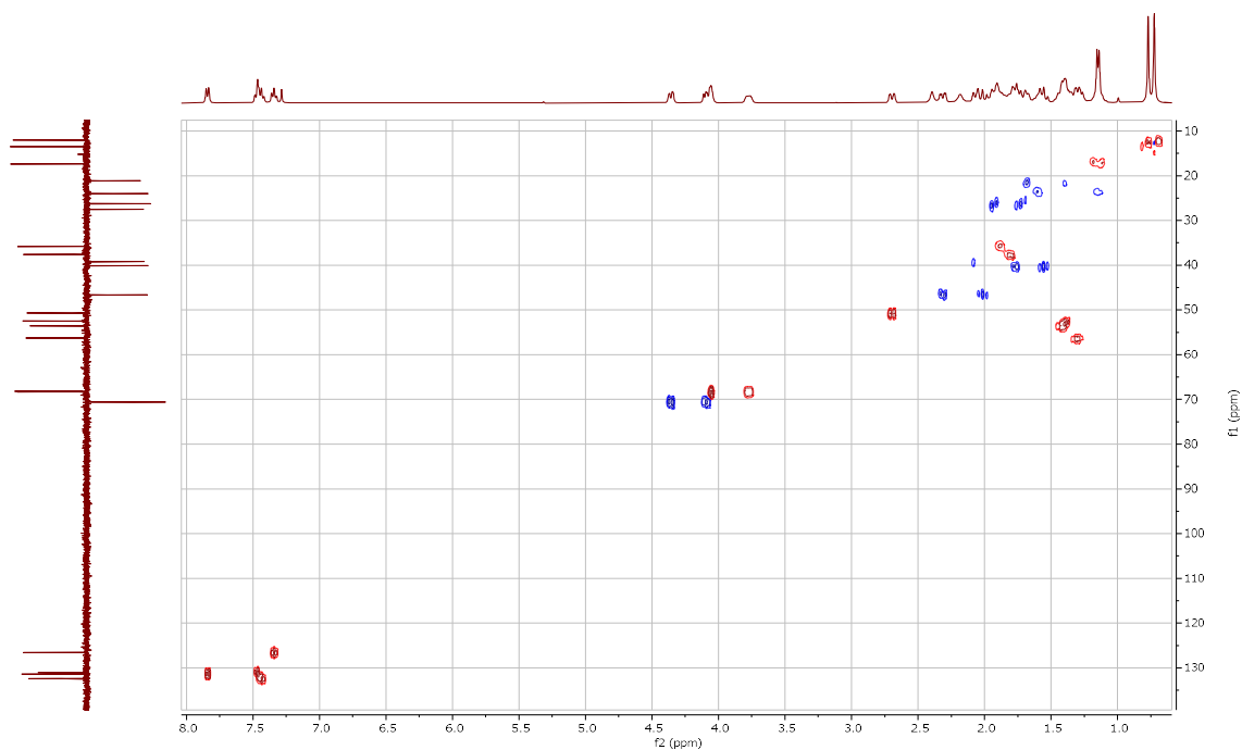
Fig. S25. 2D ^1\text{H} - ^{13}\text{C} HSQC NMR Spectrum of 2\alpha,3\alpha -Dihydroxy-6-oxo-23,24-dinor- 5\alpha -cholan-22-yl-(2-chloro)-benzoate ( 19 ).
