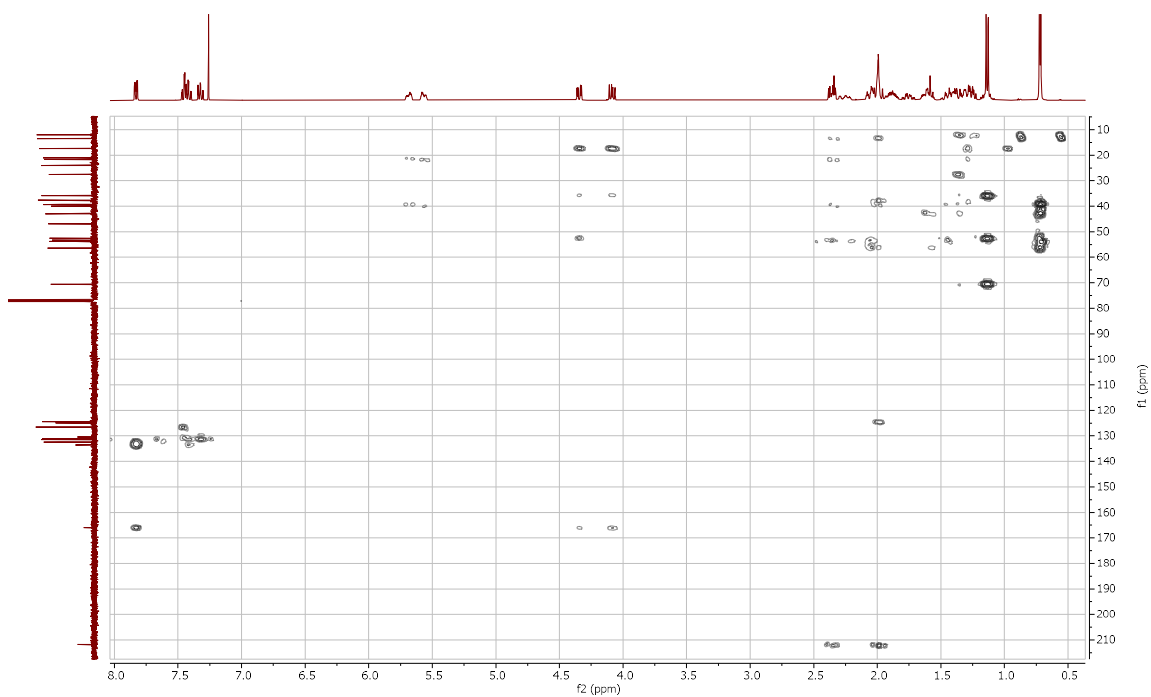
Fig. S10. 2D ^1\text{H} - ^{13}\text{C} HSQC NMR Spectrum of 6-Oxo-23,24-dinor-5 \alpha -Cholan-2-en-22-yl-(2-chloro)-benzoate (23).
