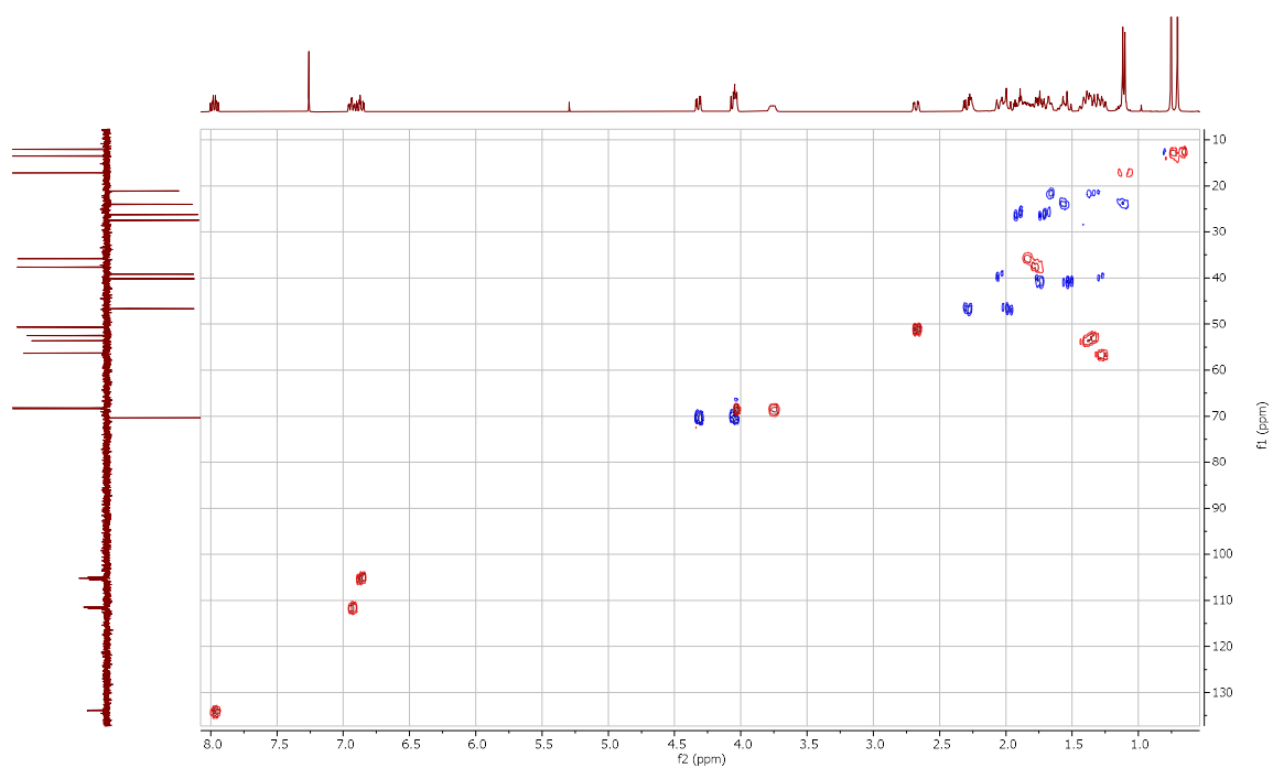
Fig. S19. 2D ^1\text{H} - ^{13}\text{C} HSQC NMR Spectrum of 2\alpha,3\alpha -Dihydroxy-6-oxo-23,24-dinor- 5\alpha -cholan-22-yl-(2,4-difluoro)-benzoate ( 18 ).
