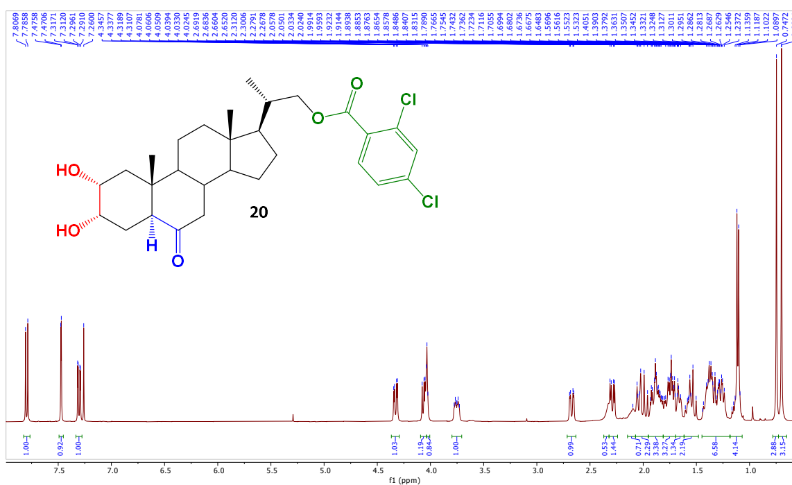
Fig. S28. ^1\text{H} NMR Spectrum of 2 \alpha ,3 \alpha -Dihydroxy-6-oxo-23,24-dinor-5 \alpha -cholan-22-yl-(2,4-dichloro)-benzoate ( 20 ).
