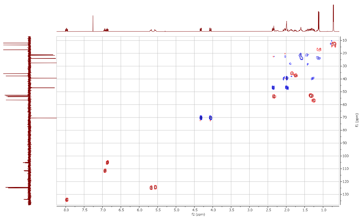
Fig. S4. 2D ^1\text{H} - ^{13}\text{C} HSQC Spectrum of 6-Oxo-23,24-dinor-5 \alpha -Cholan-2-en-22-yl-(2,4-difluoro)-benzoate (22).
