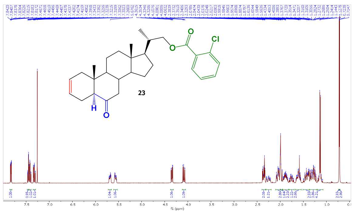
Fig. S6. ^1\text{H} NMR Spectrum of 6-Oxo-23,24-dinor-5 \alpha -Cholan-2-en-22-yl-(2-chloro)-benzoate ( 23 ).
