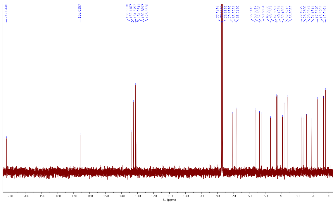
Fig. S23. ^{13}\text{C} NMR Spectrum of 2\alpha,3\alpha -Dihydroxy-6-oxo-23,24-dinor- 5\alpha -cholan-22-yl-(2-chloro)-benzoate ( 19 ).
